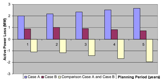
Figure 3. Comparison of active power loss between Case B and Case A
