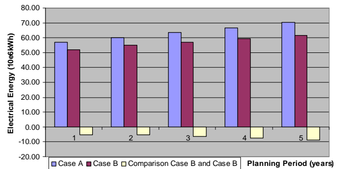
Figure 2. Comparison of electrical energy purchases from electricity markets between Case B and Case A
