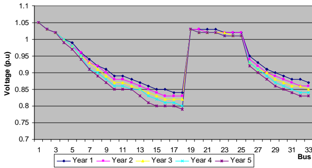
Figure 4. Bus voltage profiles in Case A
