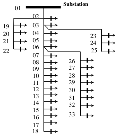
Figure 1. Diagram of 33bus IEEE radial distribution system
