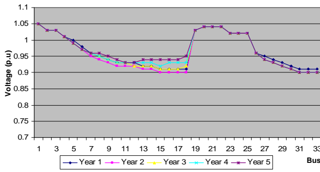
Figure 5. Bus voltage profiles in Case B
