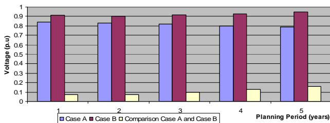
Figure 6. Comparison voltage profile of bus 18 between Case B and Case A
