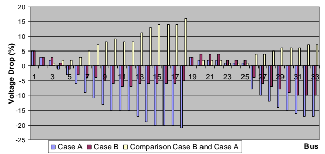
Figure 7. Comparison voltage drops between Case B and Case A
